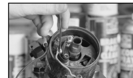
On the bench, the condenser and points come out easily. Old Autolite point sets have one hold-down screw. The breaker arm pivot slides over a support pin on the breaker plate.
