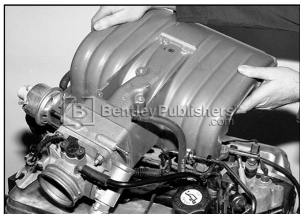
Fig. 20-3. Shown during assembly, this H.O. upper intake section still has its EGR spacer, throttle body, throttle position sensor, and EGR valve attached. Note the two center attaching bolt bosses normally hidden under the top cover plate.
