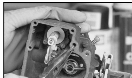
Check balls, needles and other sensitive parts need careful handling. Note that pliers grip the needle away from the tapered tip.
