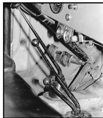
Mechanical clutch linkage requires regular inspection for wear and excessive play. Models with through-the-floor pedals have the advantage of chassis mounted linkage. This reduces the tendency to flex, distort and bind.
