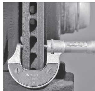
Measuring brake rotor wear. 00.04 Maintenance
