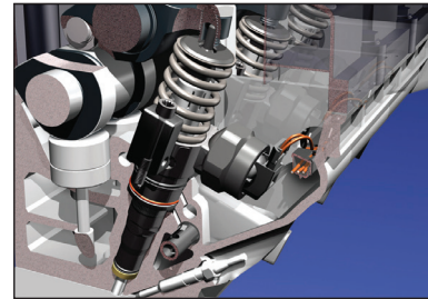
Pumpe Düse pump injector overview Product Familiarization
