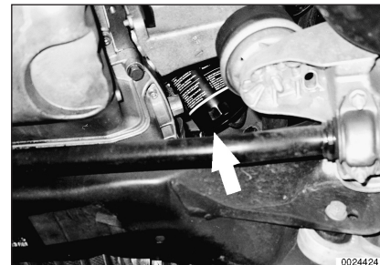
Engine oil and filter changing procedures, including filter location Section A - Maintenance
