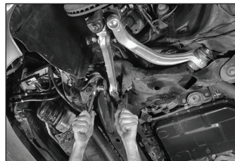
Step-by-step front suspension component replacement. 40 Front Suspension
