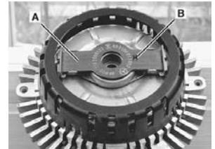
Learn how to cure a hot-running V-8 engine by modifying the viscous fan clutch. Chapter 5: V-8 Engine
