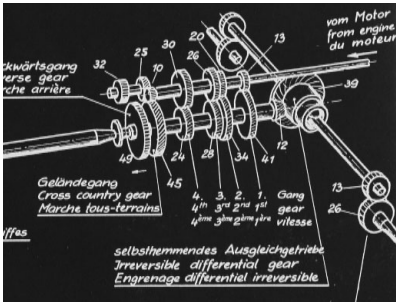
Chapter 8: The drive train for the Hunter included a clutch that allowed drive to the front wheels to be engaged or disengaged by the driver.
