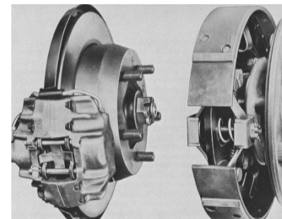
Chapter 11: The Porsche-Ate disc brake (left), as fitted to the 356C. At right is the hand brake.
