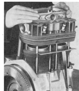
Removing and Installing Cylinder Head, Section M, Engine and Clutch
