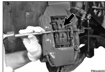
Step-by-step brake pad and rotor replacement. 46 Brakes—Mechanical
