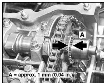
Engine and cylinder head service, including Double VANOS timing chain setup and adjustment. 117 Camshaft Timing Chain
