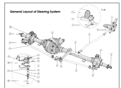
Steering linkage: When servicing the steering system, steering linkage requires attention. The linkage consists of a draglink, bellcrank, tie-rods and the attaching tie-rod joint ends. Wear occurs at any of the pivotal points in the joints.
